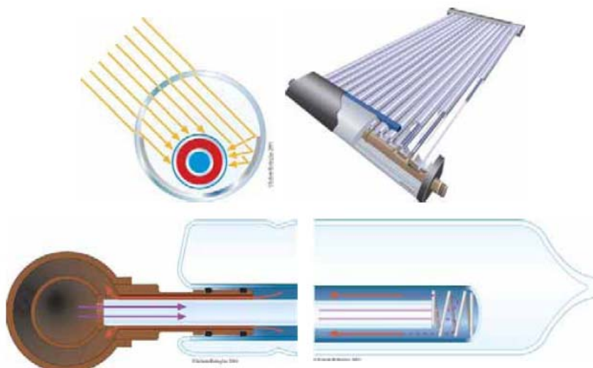
Figura 3.16 - Tubo colector Schott
